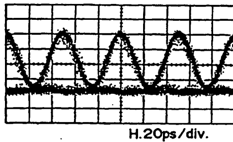
② 20 Gb/s OPTICAL RZ WAVEFORM
